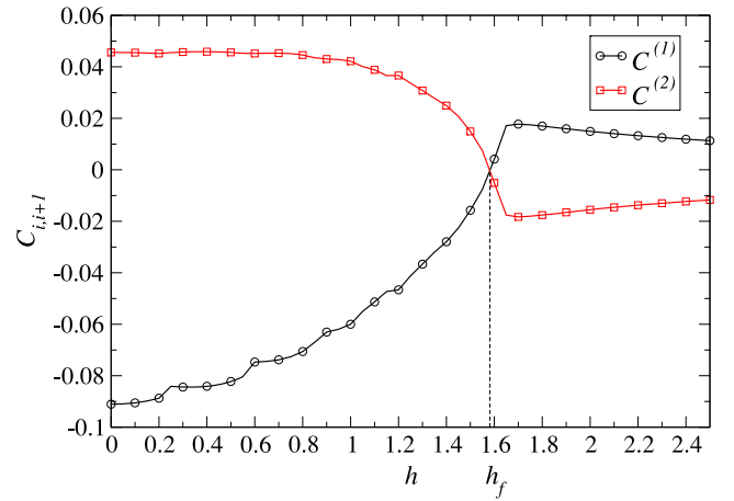
Figure 2. Entanglement estimators of the XXZ spin-1/2 chain versus transverse field h with parameter \Delta = 0.25 . C^{(1)} is depicted by (black) circles and C^{(2)} by (red) squares. At the classical field ( h = h_f \simeq 1.58 ), C_{i,i+1}^{(1)} = C_{i,i+1}^{(2)} = 0 .
